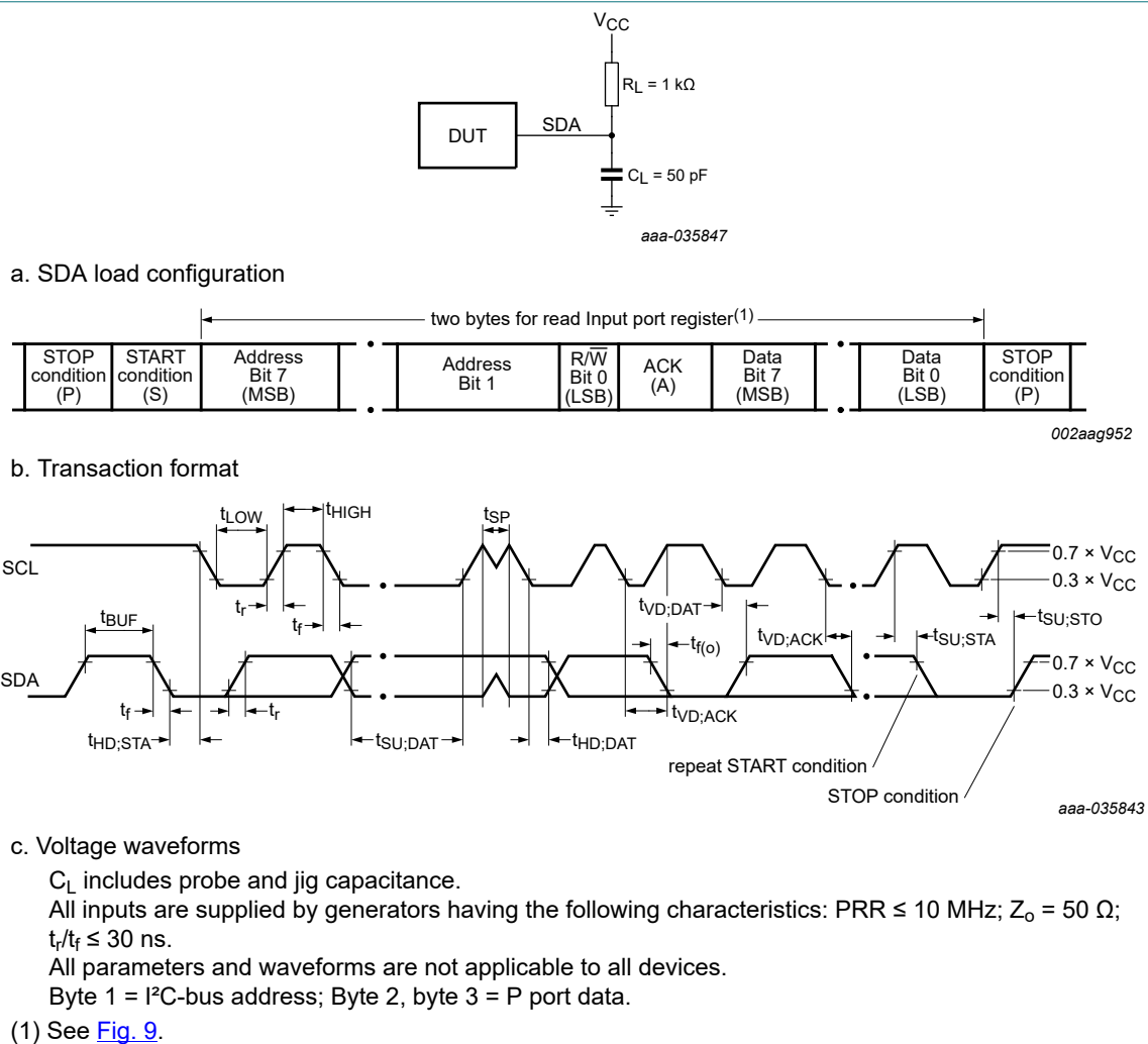
Fig. 26. I 2 C-bus interface load circuit and voltage waveforms
