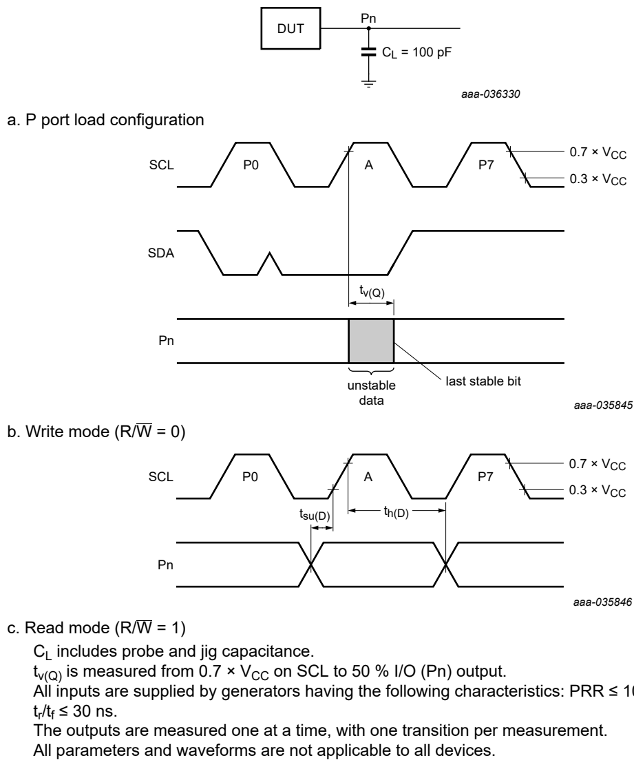
Fig. 28. P port load circuit and voltage waveforms
